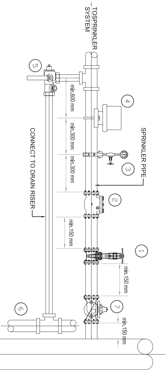
COMBINATION STANDPIPE RISER
